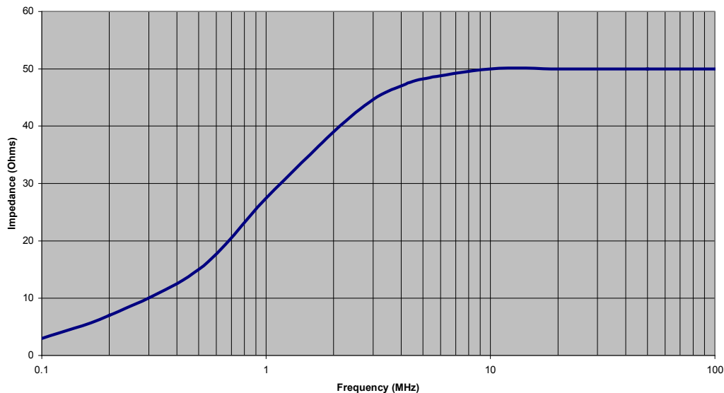
CISPR25 Impedance characteristic
