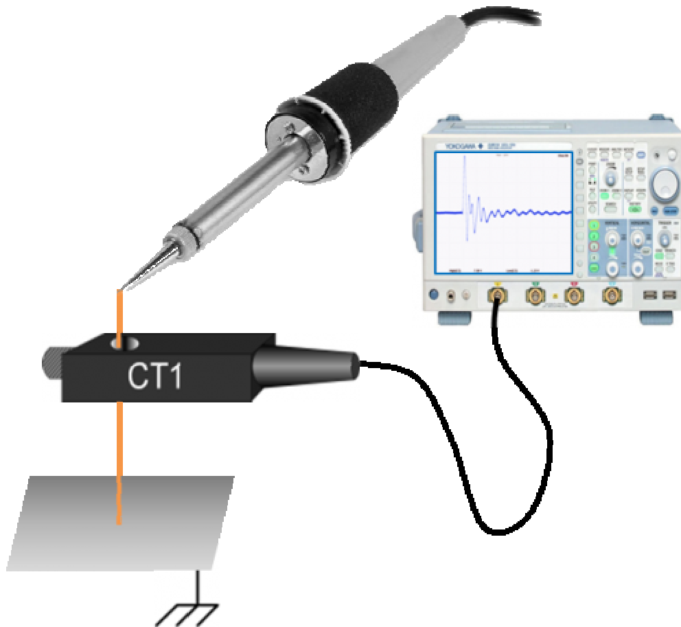
Figure 3 Test Setup for Measuring EOS Exposure
