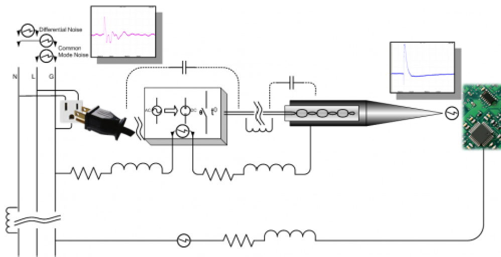
Figure 5 Noise Propagation in the Soldering Iron
