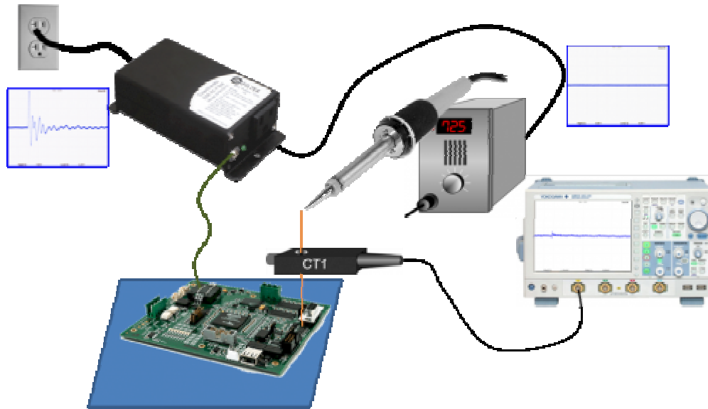
Figure 7 Soldering Iron with Power Line EMI Filter (OnFILTER model APN515LG)
